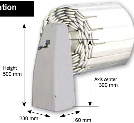
Electric box for 24V motor
